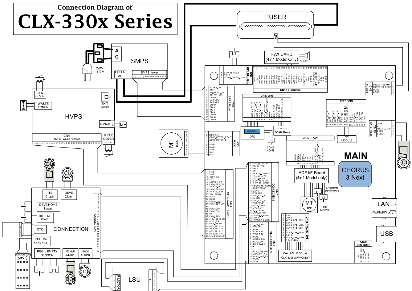
Diagram of the CLX-330x series Electrical Circuit
